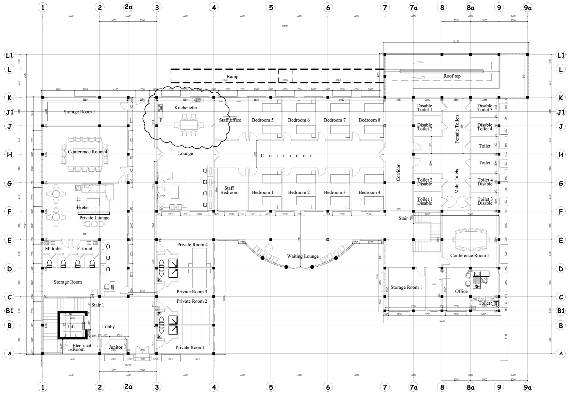
SECOND FLOOR PLAN SCALE: 1:100
