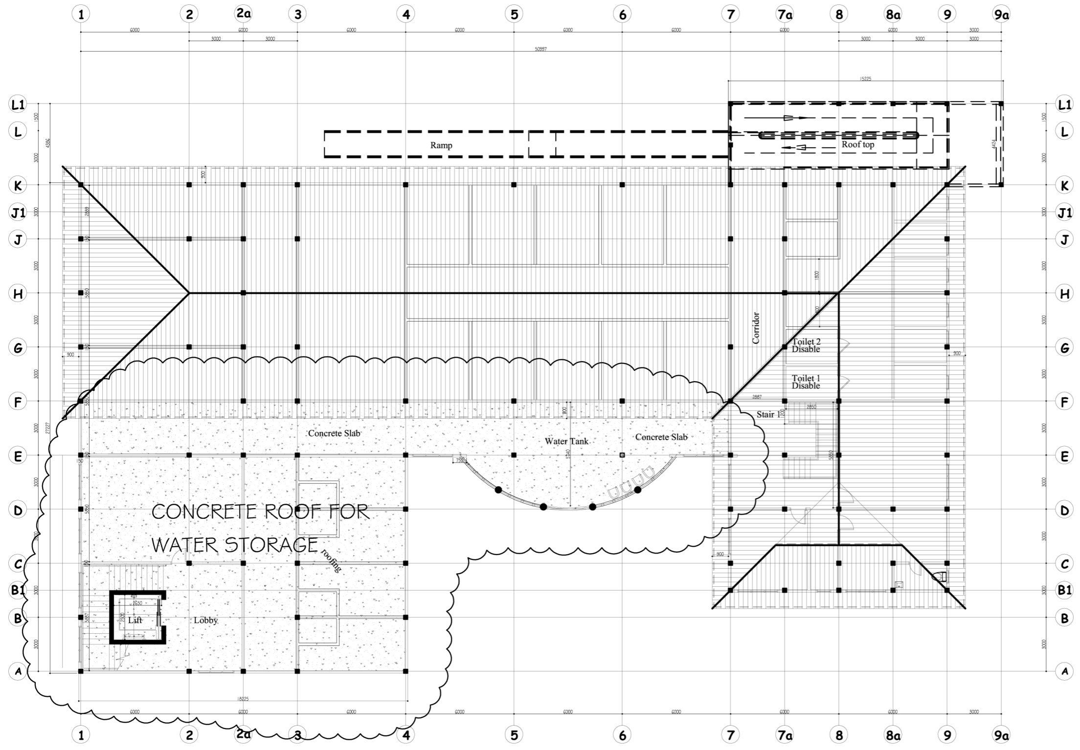
UPPER ROOF PLAN SCALE: 1:100
