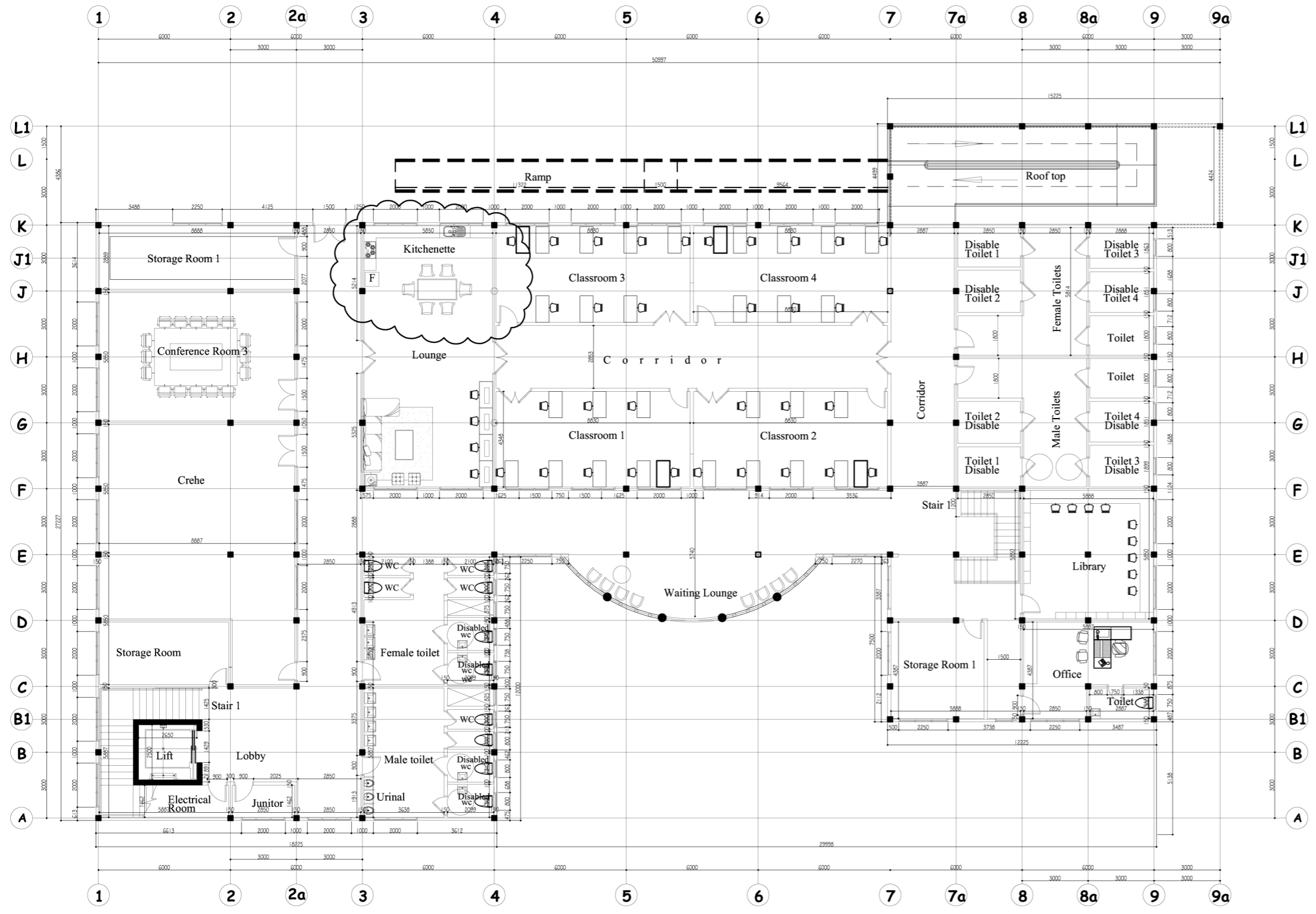
FIRST FLOOR PLAN SCALE: 1:100
